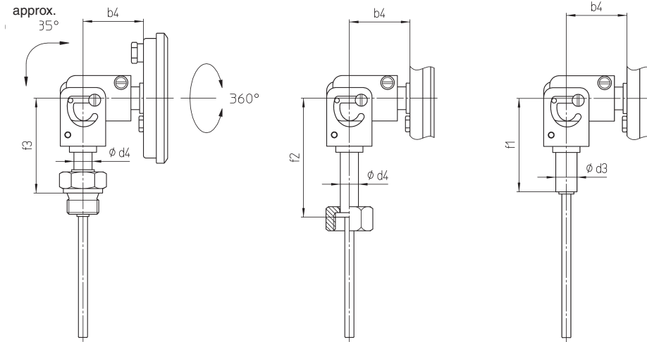
Stem type B4.1, rigid male connection
