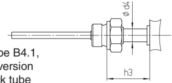
Stem type B4.1, standard version without neck tube
