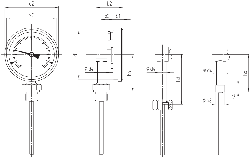
Stem type B4.1, rigid male connection
