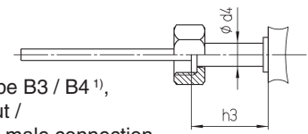
Stem type B4.1, special version with neck tube
